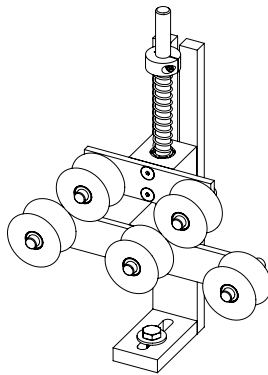
40-4335 SPRING PRESSURED INCOMING GUIDE ROLL ASSEMBLY
