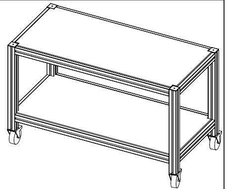
41-1071 DUAL PRINTER STAND
