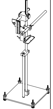
50-1003 TWO HEAD BOOM STAND FOR TOP AND BOTTOM PRINTING
