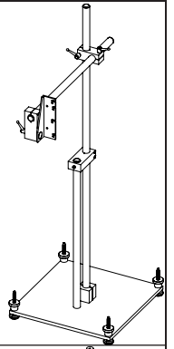
41-1059 SINGLE HEAD BOOM STAND
