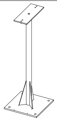
98-0221 PEDESTAL STAND 10" BASE
