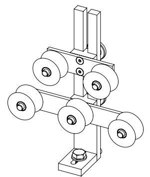
98-0076 INCOMING GUIDE ROLL ASSEMBLY
