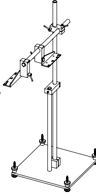
50-0062 TWO HEAD BOOM STAND FOR SIDE PRINTING
