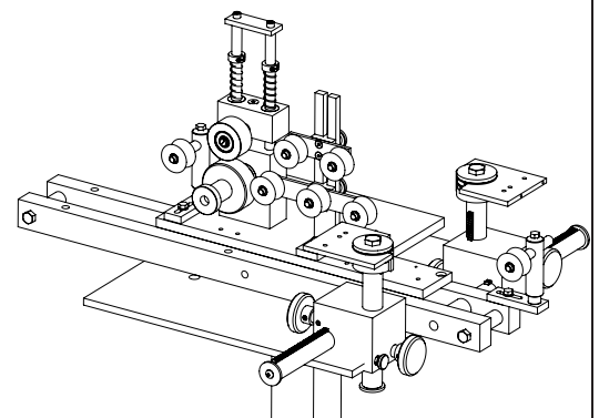
98-0247 WIRE MANUFACTURING GUIDE W/DUAL XY HEADS ON HD STAND
