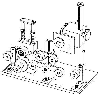
98-0059 WIRE MANUFACTURING GUIDE
